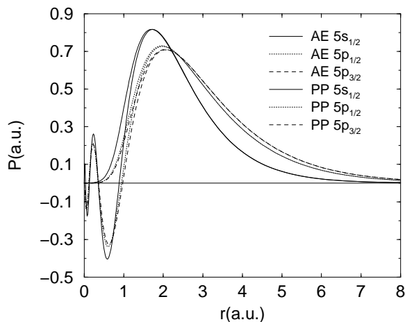
Figure 6. Valence spinors of the iodine atom in the [_{46}\text{Pd}] 5s^2 5p^5 ground state configuration from average-level all-electron (AE) multiconfiguration Dirac-Hartree-Fock calculations and corresponding valence-only calculations using a relativistic energy-consistent 7-valence-electron pseudopotential (PP).
