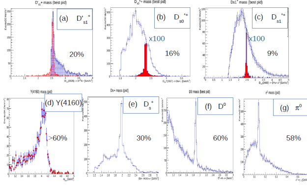
Fig. 22: Invariant mass distributions of the decay particles of (a) D'_{s1}(2536)^+ (b) D_{s0}(2317)^{++} (c) D'_{s1}(2460)^{++} (d) Y(4160) \rightarrow e^+e^- (e) D_s^+ (f) D^0 \rightarrow K^+K^- (g) \pi^0 \rightarrow \gamma\gamma . The reconstruction efficiency values are shown in the figures, respectively.
