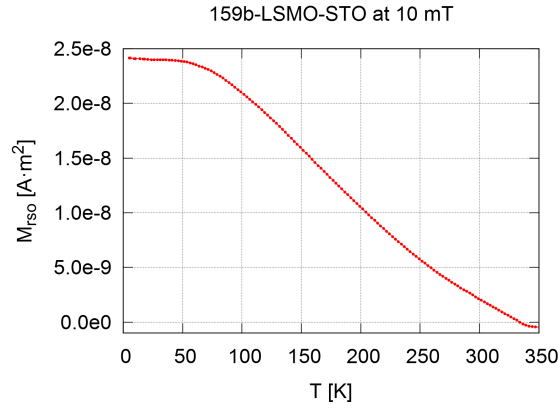
(c) Magnetic characterization of post-annealed sample 159b: Smeared out Curie temperature
