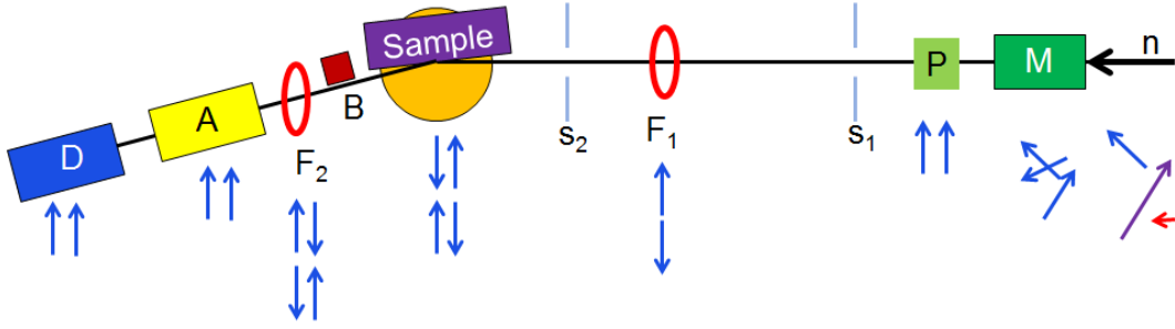
Figure 3.6: Components of a polarized neutron reflectometer: The neutron beam passes a mochochromatizer (dark green), a polarizer (light green), 2 slits ( s_1 and s_2 , a flipper (red circle), the sample stage (orange) including magnet, cryostat and sample (violet), a beamstop (red rectangle), a second flipper (red circle), an analyzer and is stopped by the detector (blue rectangle). For details, see text.
