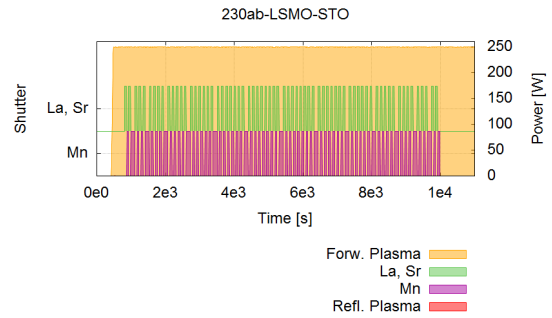
(b) Logfile 230 (edged Mn excess)
