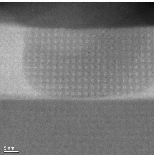
(e) Other defect zone: Perfect perovskite structure
