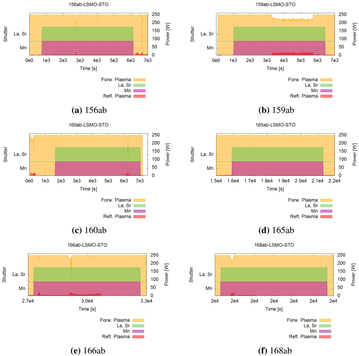
Figure C.4: Logfiles of sample series 156ab-168ab during growth
