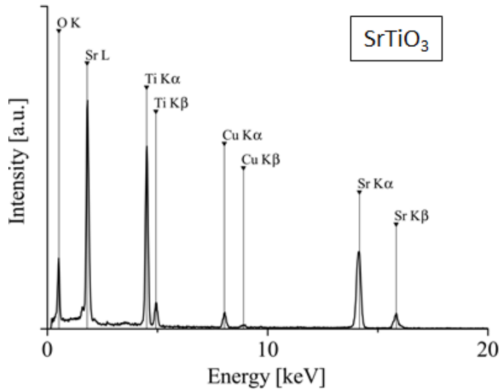
(b) EDX spectrum of substrate
