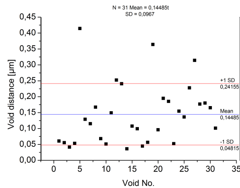
(c) Distance between neighboring voids
