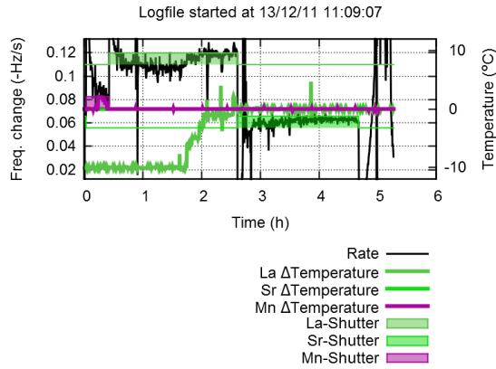
(c) Logfile 230 calibration
