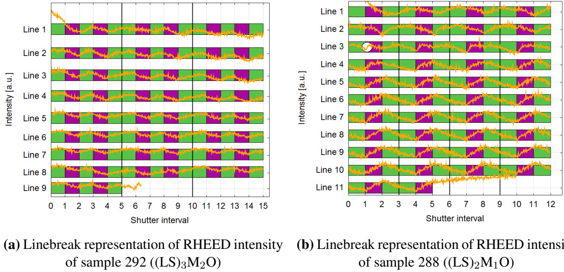
Figure 6.2: LS_3M_2O and LS_2M_1O : RHEED linebreak visualization
