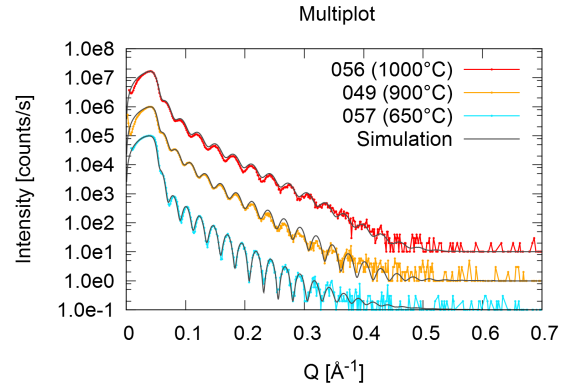
(b) XRR of samples 057 (650 °C), 049 (900 °C), 056 (1000 °C)
