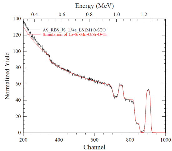
(f) RBS of sample 134a
