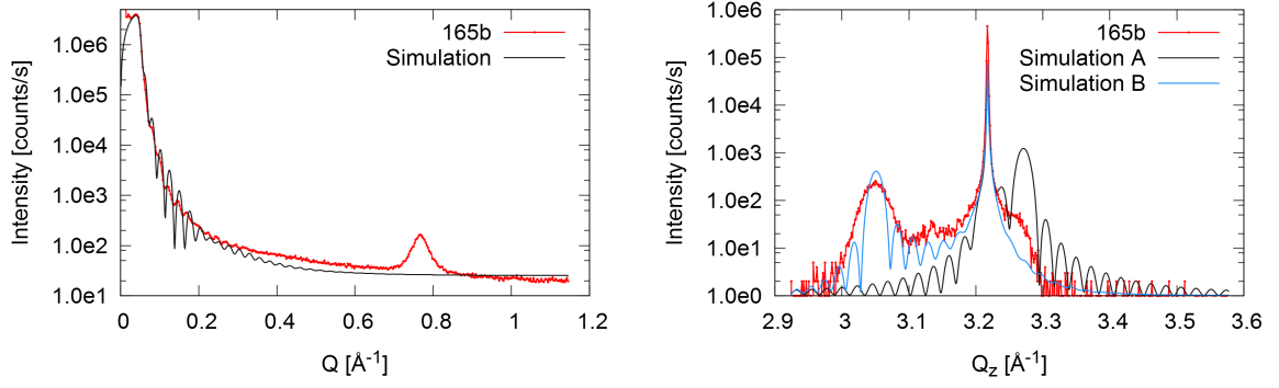
(a) XRR of sample 165b after post-annealing: Extremely rough surface (b) XRD of sample 165b after post-annealing: Shifted layer lattice parameter
