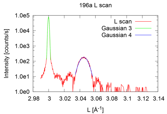
(f) Line scan along L through substrate and layer peak
