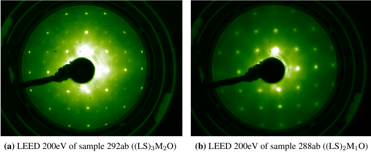
Figure 6.3: LEED performed at samples 292ab and 288ab
