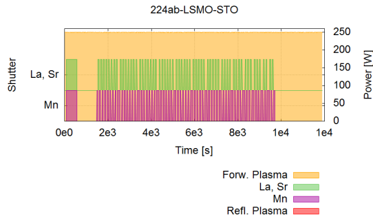
(a) Logfile 224 (top Mn excess)
