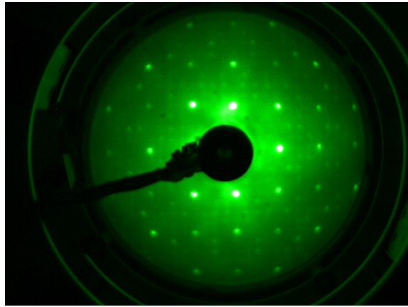
(b) LEED at 200 eV of sample 134ab
