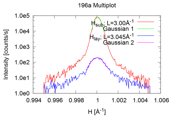
(e) Line scans along H through substrate and layer peak
