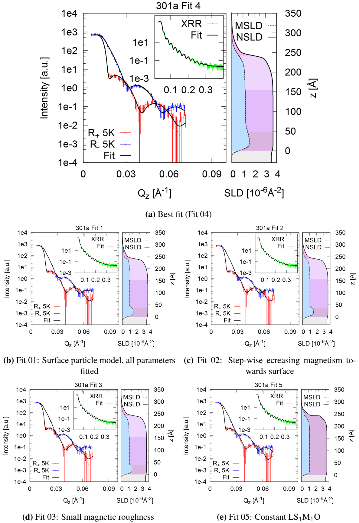
Figure 7.5: Comparison of influence of different models for fitting the 301a measured at TREFF@MLZ
