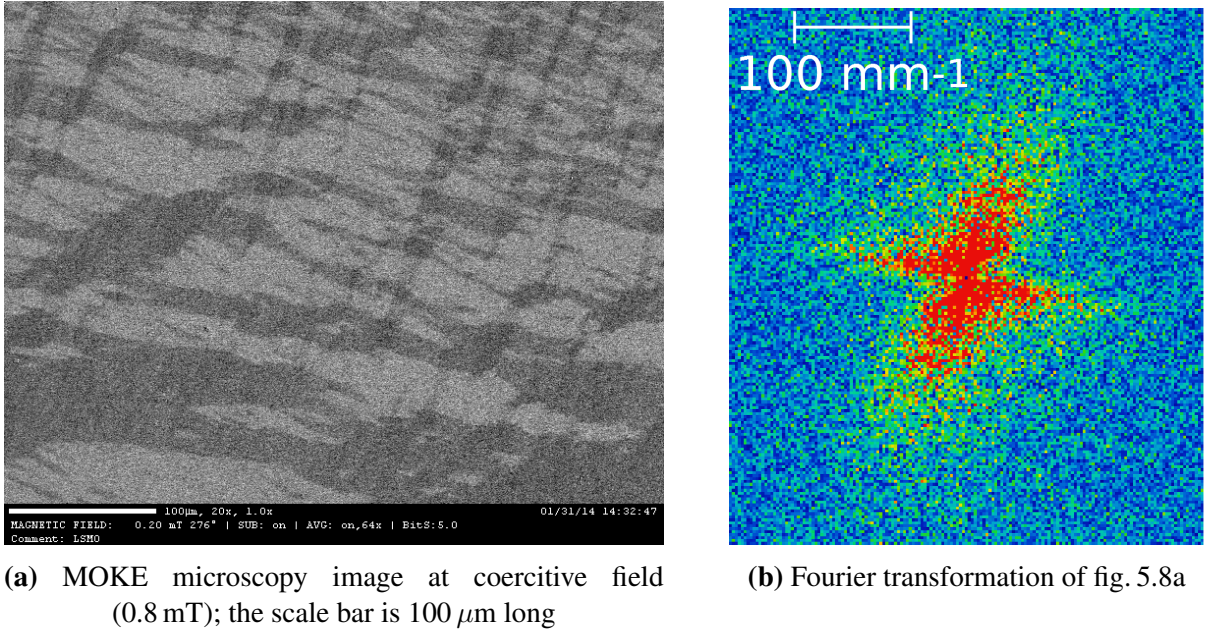
Figure 5.8: MOKE image of sample 196b
