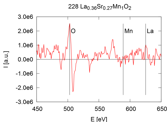
Figure 3.3: AES spectrum of sample 228: Indeterminable La/Mn ratio
