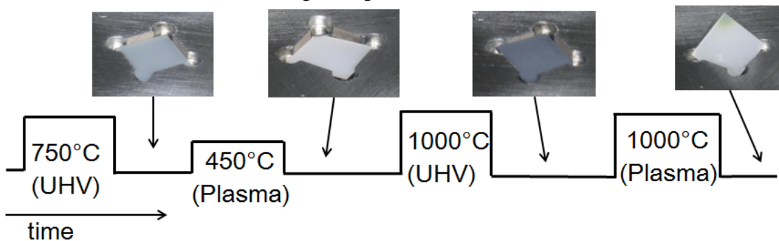
(b) STO substrate was heated several times, either in UHV or in oxygen plasma: The \text{SrTiO}_3 color changes are reversible
