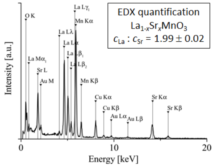
(a) EDX spectrum of layer
