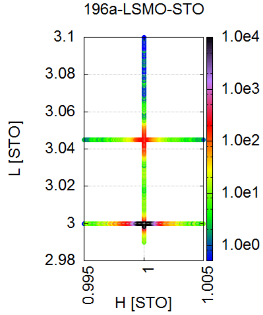
(b) line scans of region of fig. 5.7a. Position, size and shape of layer as well as substrate peak can be identified
