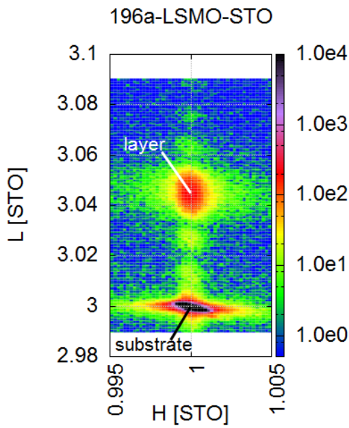
(a) XRD map around (1 0 3) substrate peak - epitaxial layer growth due to identical in-plane parameter of substrate and layer
