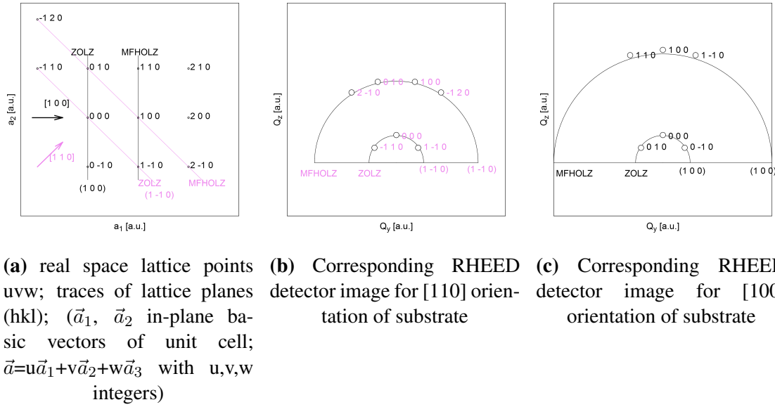
Figure 3.4: RHEED indexing
