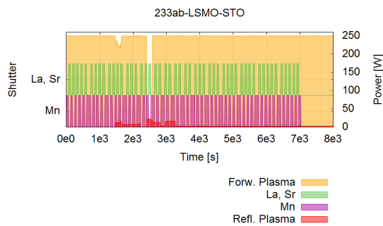
(c) Logfile 233 (centered Mn excess)
