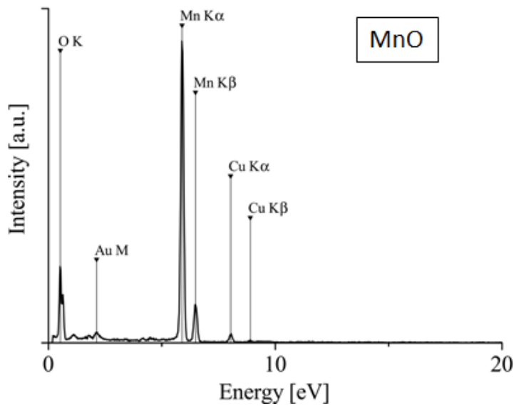
(c) EDX spectrum of precipitate
