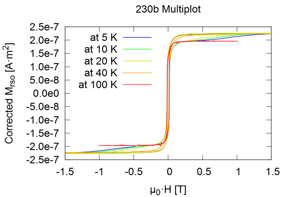
(e) Multiple hysteresis loops
