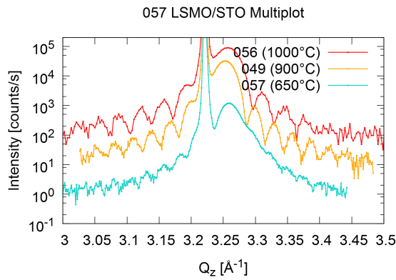
(c) XRD of samples 057 (650 °C), 049 (900 °C), 056 (1000 °C)
