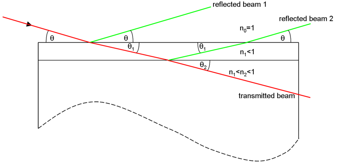
Figure 2.4: Reflection and refraction from a single layer on a substrate; incoming beam in red, reflected beam in green. Taken from [24]
