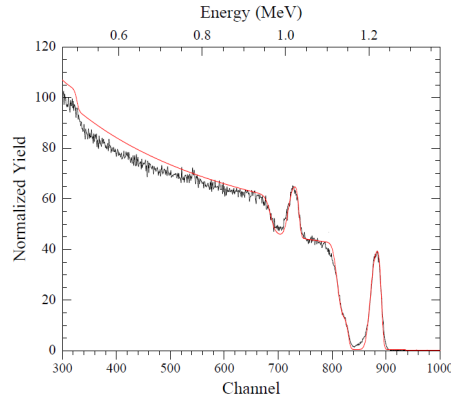
Figure 8.5: RBS data and simulation of sample 301a
