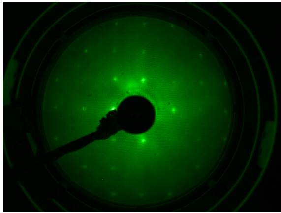
(a) LEED of sample 049 (900 °C)
