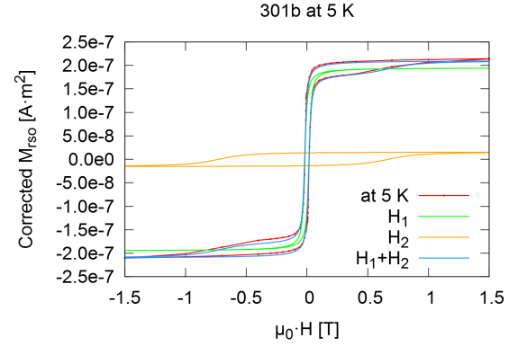
(b) 301b: Hysteresis loop at 5K
