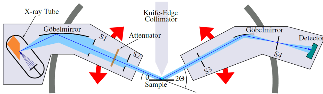
Figure 3.5: XRR sketch, taken from [51]
