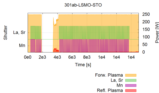
(e) Logfile for 301ab
