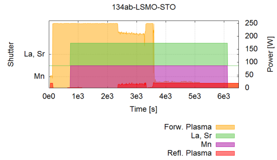
(b) Sample 134: Logfile during growth
