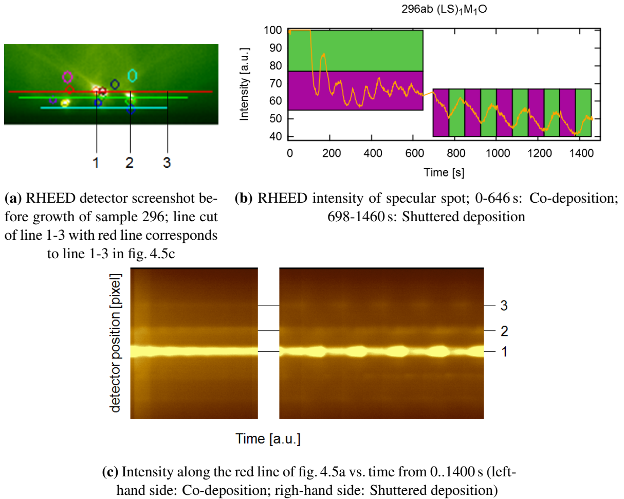
Figure 4.5: Calibration procedure for shuttered growth deposition
