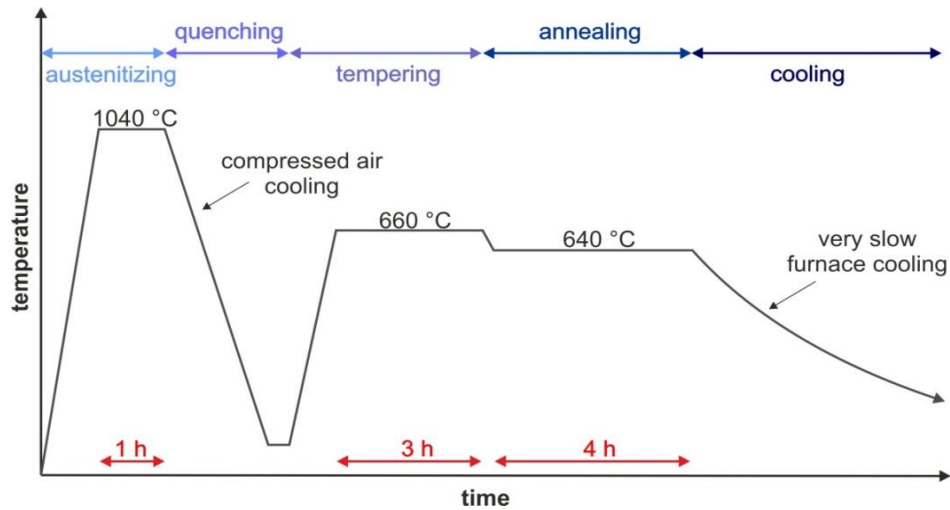
Image 2: The heat treatment scheme of X10CrNiMoV12-2-2 Steel
