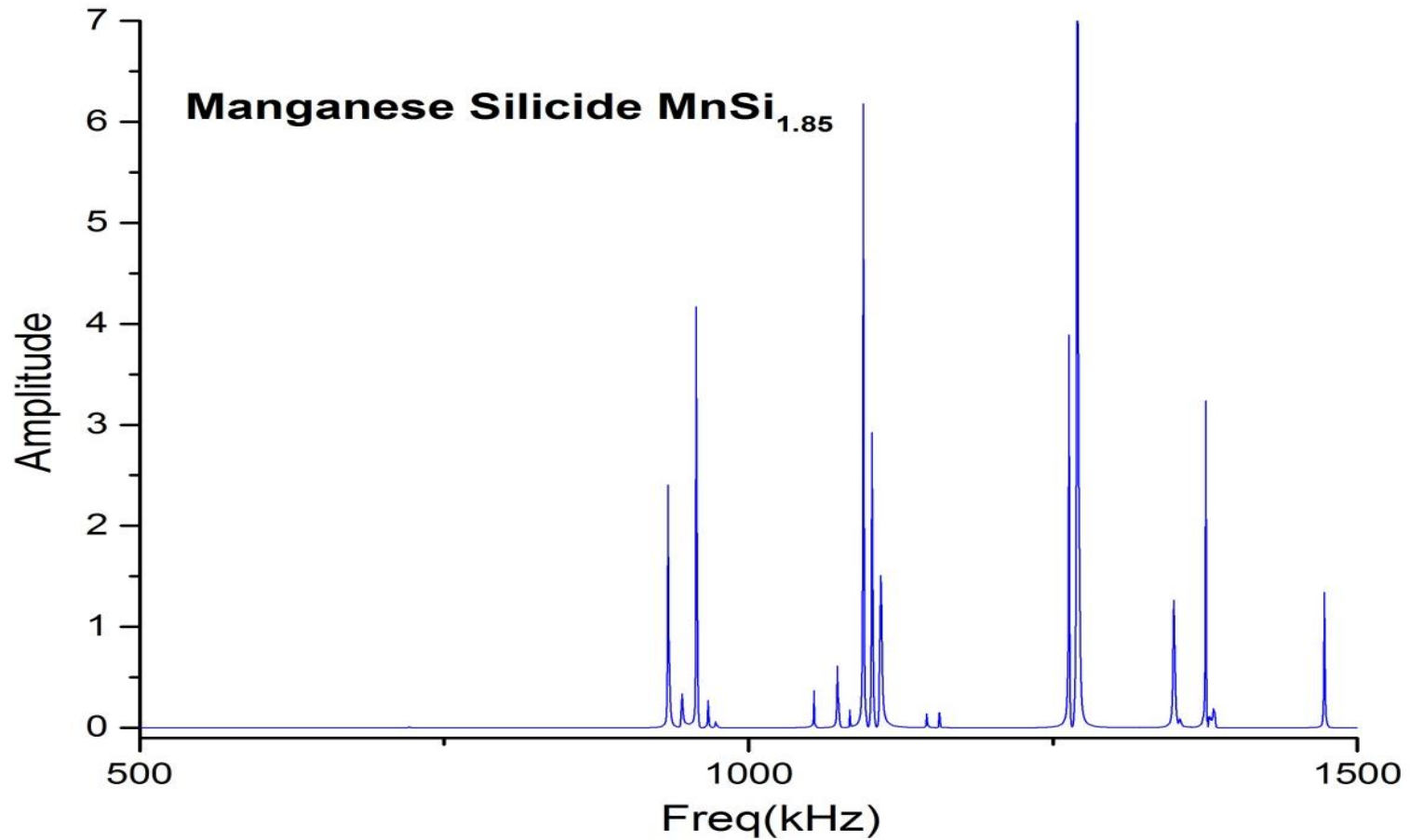
Image 63: Resonance profile of \text{MnSi}_{1.85}
