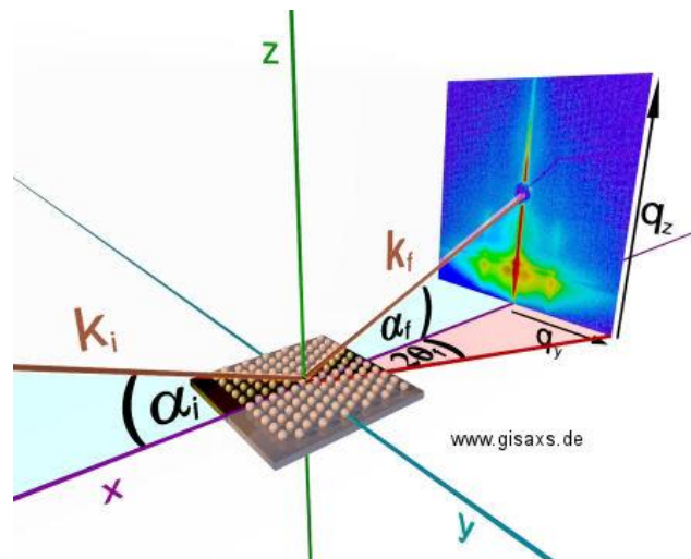
Image 19: GISAXS geometry [Mey12]
