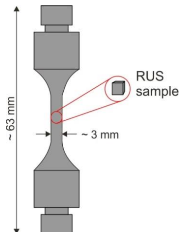
Image 32: Schematic profile of RUS specimen
