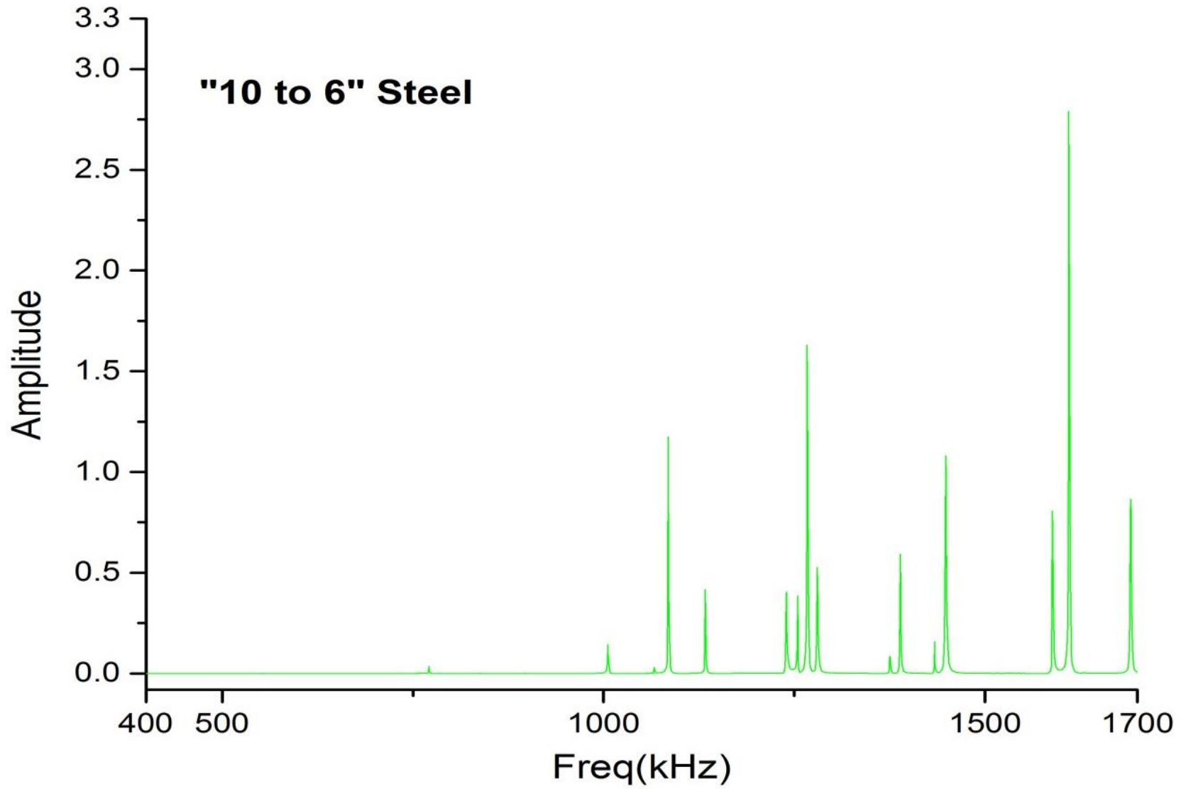
Image 65: Resonance profile of "10 to 6" steel
