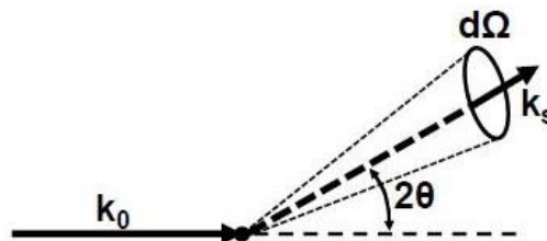
Image 17: Schematic image of solid angle d\Omega
