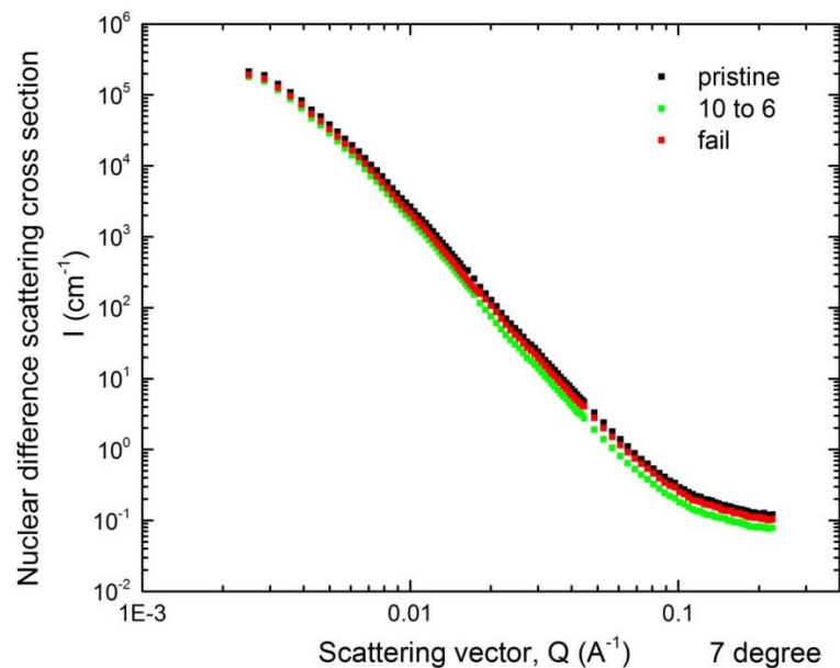
Image 44: Nuclear components of SANS profiles obtained from "pristine", "10 to 6" and "fail" steel with \Phi = 90 \pm 7^\circ angle mask
