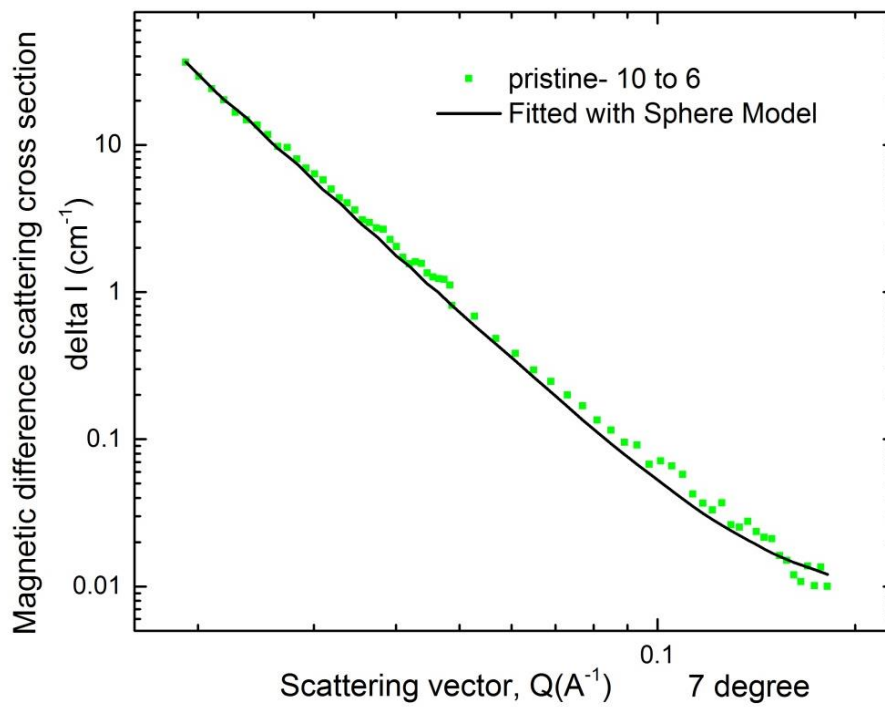
Image 57: SANS sphere model of "pristine-10 to 6" at 7-degree magnetic mask.
