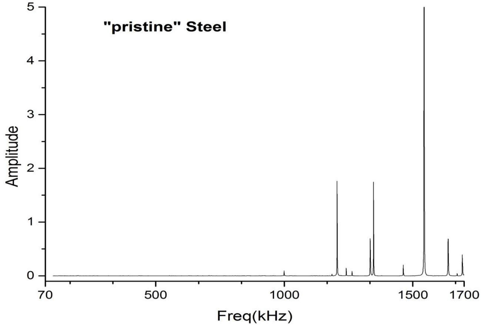
Image 64: Resonance profile of "pristine" steel
