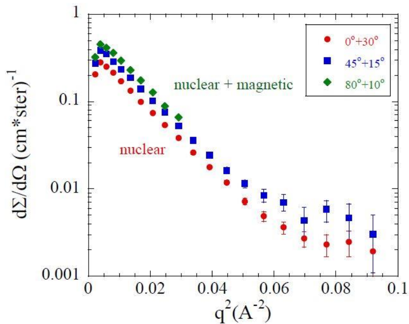
Image 13: The scattering differs from the angle [Koh97].
