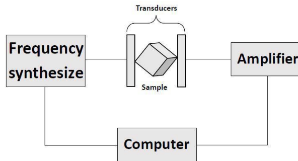
Image 21: The basic model of resonant ultrasound spectroscopy
