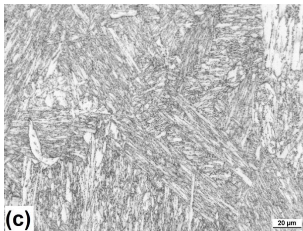
Image 41: Microstructures of: (a) "pristine"; (b) "10 to 6"; (c) "fail" specimens
