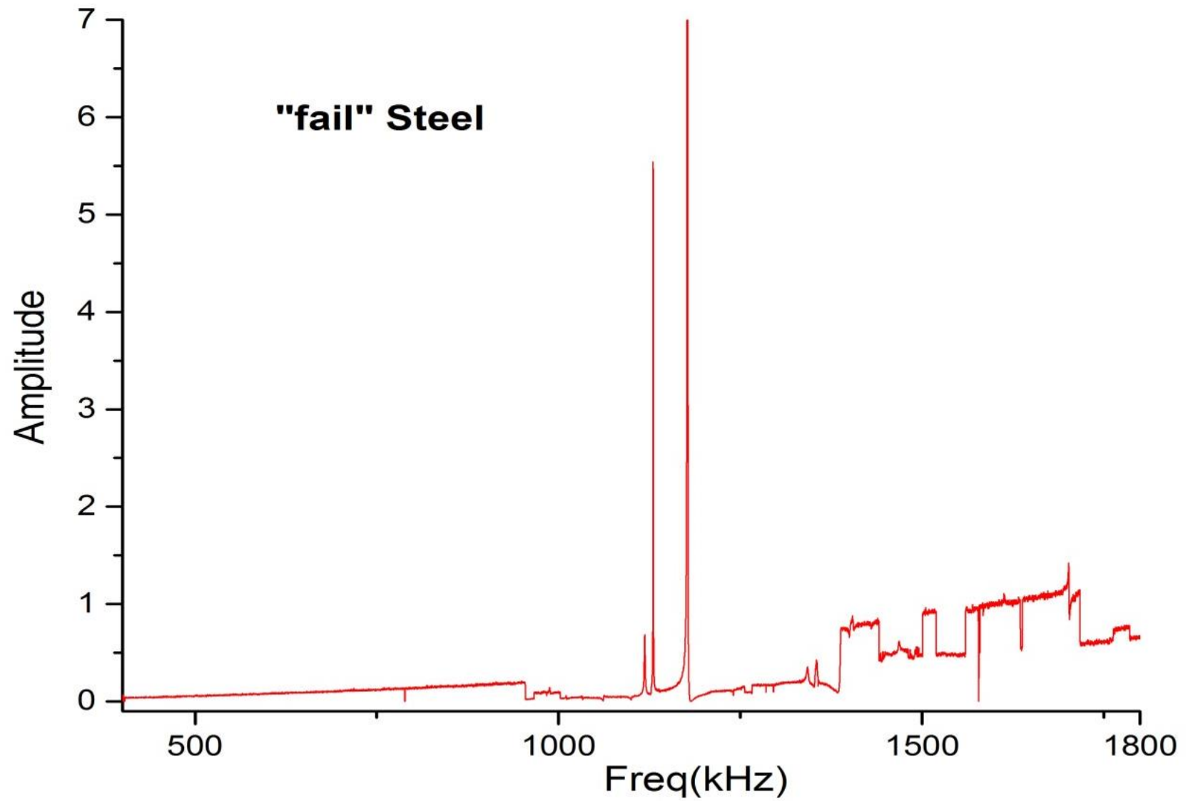
Image 66: Resonance profile of "fail" steel
