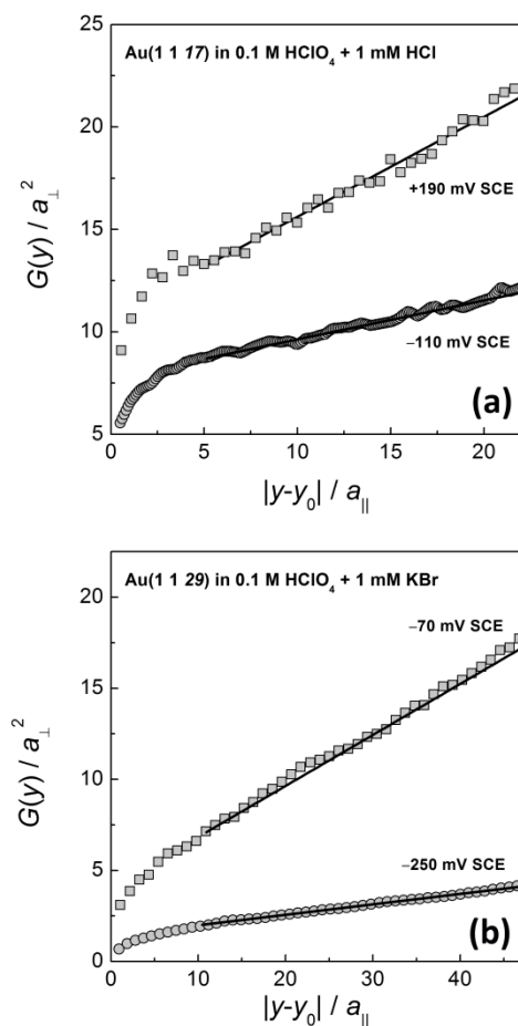
Fig. 3: Spatial correlation function G(y) (eq. (1)) for (a) Cl - and (b) Br - containing electrolyte at different potentials. Solid lines are linear fits to the curves in the range of large distances (see text for further discussion).
