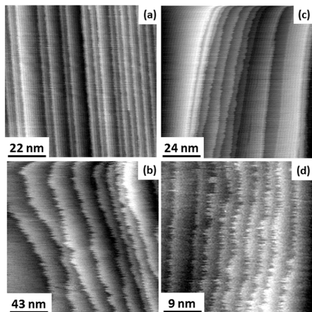
Fig. 1: STM images of Au electrodes in 0.1 M HClO 4 + 1 mM HCl (a) (1 1 29) at -0.17 V SCE, (b) (1 1 17) at +0.45 V SCE and in 0.1 M HClO 4 + 1 mM KBr (c) (1 1 29) at -0.25 V SCE, (d) (1 1 29) at +0.31 V SCE.
