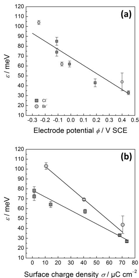
Fig. 4: (a) Kink energy as determined from experimental data for G(y) (eq. (1)) similar to those presented in Fig. 3 for Cl - (dark grey squares) and Br - (light grey circles) containing electrolyte vs. electrode potential. (b) The same data plotted vs. surface charge density taken from Fig. 2(b). Solid lines are linear fits to the data (see text for further discussion). Error bars are determined as the standard deviation from the mean for independent measurements at the same electrode potential.
