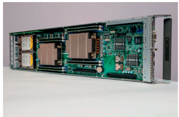
View of a T-Platforms V-Class V210S dual-socket blade server as used in JURECA.
