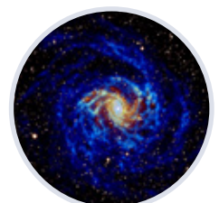
Radio Astronomy
