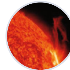
Space Weather
