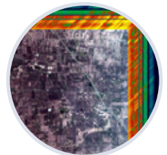
Earth Science
