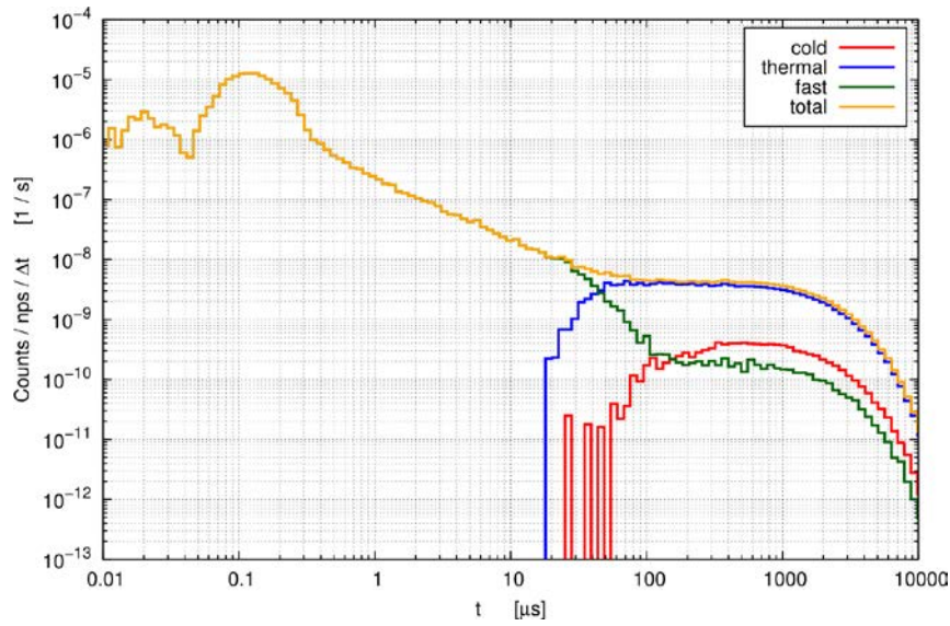
Fig. 10. Pulse shape of neutrons leaving the moderator at the channel opening. Neutrons with energy below 13.1 meV (150 K) are referred to as cold neutrons, below 127 meV (1474 K) thermal neutrons and above fast neutrons.
