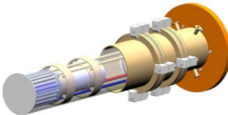
Fig. 15. Cold source prototype as developed and built for tests at the AKR-2. The cold source is a cylindrical Al vessel ( r=25 mm, l=100 mm) to condense H_2 or CH_4 gas, surrounded with a He gas cooling labyrinth. The working pressure is defined as 1.5 bar for liquid H_2 . The cold source is installed on a standard flange and can be inserted into an evacuated beam tube in the thermal moderator. 4 gas connections are used for input and output of moderator gas and He cooling gas. On the moderator surface towards the opening of the beam tube, a filter crystal can be mounted for further treatment of the spectrum.
