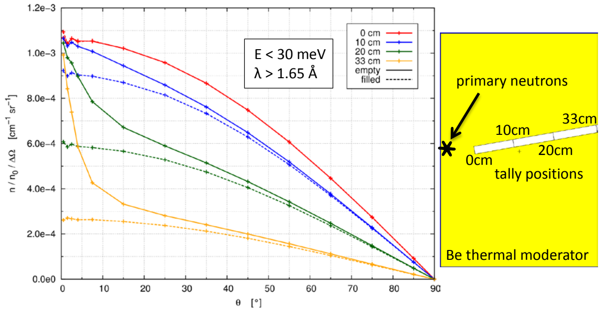
Fig. 7. Left: Angular distribution of neutrons passing a surface inside a channel at various depths for the case of an evacuated channel and a filled channel, respectively. The position at 0 cm corresponds to the bottom of the channel, while 33 cm denotes its opening. Solid lines indicate evacuated channel and dashed lines represent filled channel. Right: Corresponding MCNP geometry (cut through a cylinder). The source of primary neutrons is located on the left surface of the moderator cylinder. A vacuum channel with r = 2 \text{ cm} is implemented at the right moderator surface originating at the thermal flux maximum with a 10^\circ inclination. Detector areas are defined at different depths inside the vacuum channel.
