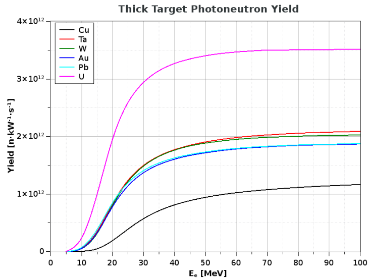
Fig. 3. Neutron yield (per kW power of an electron accelerator) for different materials for an electron beam as a function of the electron energy.
