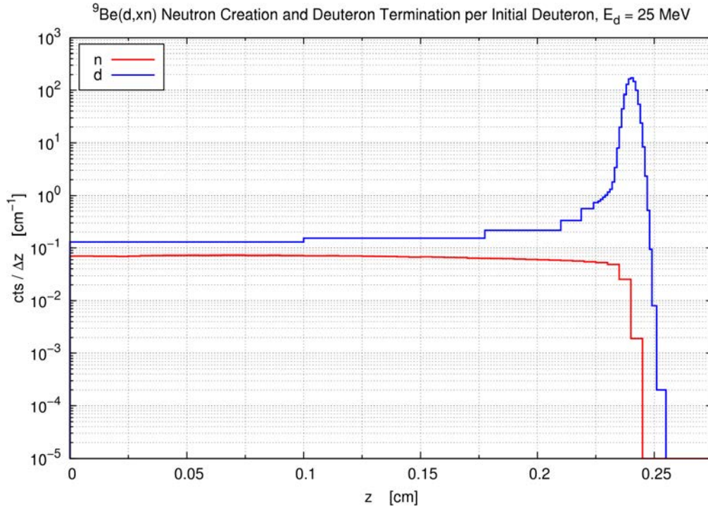
Fig. 5. Depth dependence of neutron production and D^+ ion stopping probability for a 25 MeV deuteron beam on a bulk Be target. 99% of primary neutrons are produced up to a penetration depth of 0.225 cm while 0.2% of deuterons are deposited.
