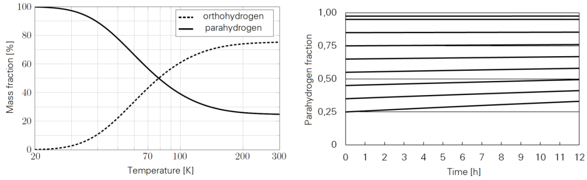
Fig. 13. Temperature dependent thermodynamic equilibrium of ortho- to para-hydrogen mixtures (left) and change of hydrogen composition due to auto conversion over 12 hours in liquid hydrogen at 17 K and 0.15 MPa (right).
