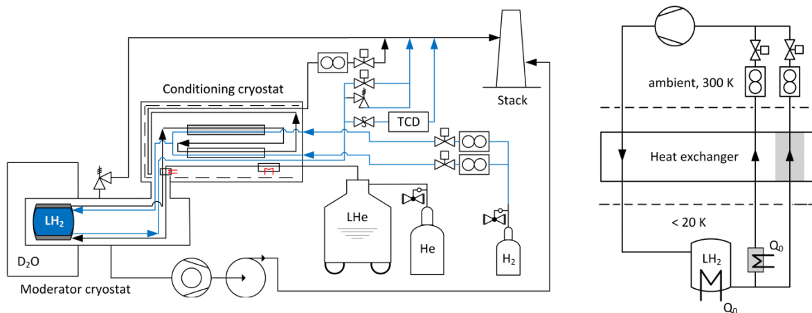
Fig. 14. Setups with adjustable ortho- to para-hydrogen composition for proof of principle (left) and for a closed hydrogen system for a HBS facility (right). The moderator vessel (ca. 0.3 liters LH 2 ) will be cooled externally by a helium cold gas to 17 K. Two tube in tube heat exchangers cool down
