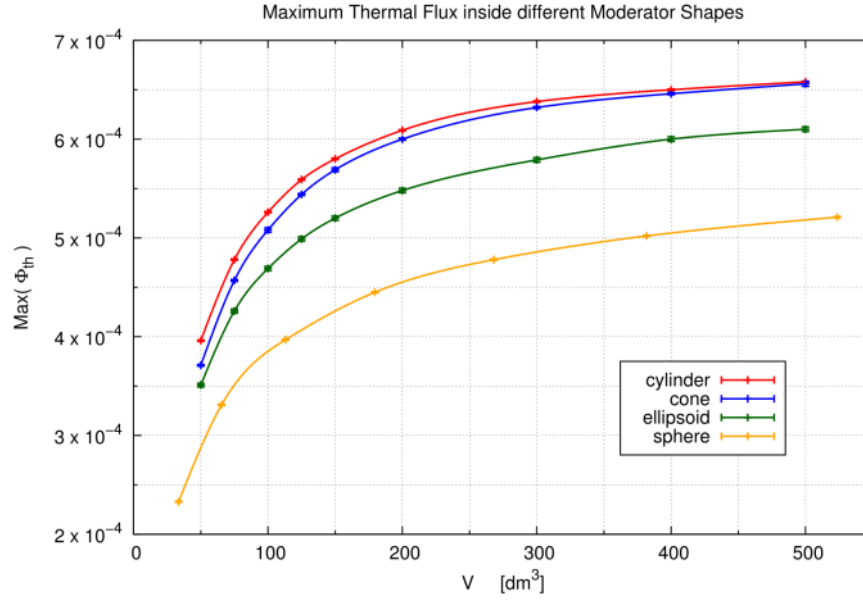
Fig. 6. Maximum thermal flux normalized to the number of primary neutrons depending on the volume of spherical, cylindrical, conical and elliptical beryllium moderators. The axes of symmetry of the moderator geometries and the beam direction of the source particles point in positive z-direction. Since the volume of the latter three depends on two parameters, only the optimal parameter combination for a given volume is plotted.
