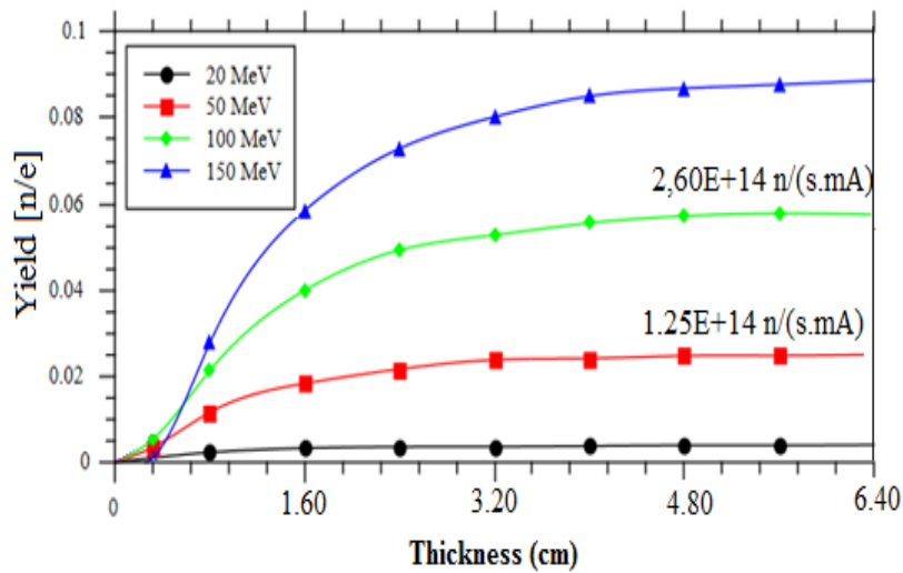
Fig. 4. Simulation of the neutron yield (per incident particle) for a uranium target for different electron energies as a function of target length.
