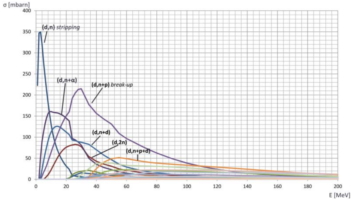
Fig. 1. Energy dependence of the cross sections of different neutron emitting reactions for deuterons impinging on Be.
