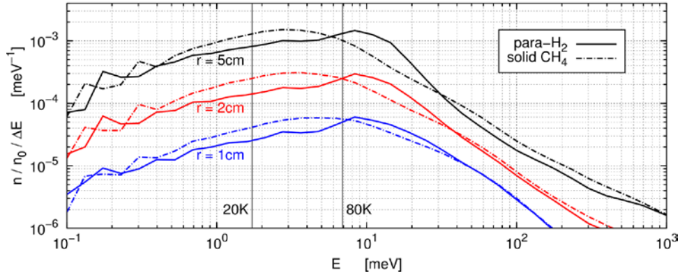
Fig. 12. Spectrum of neutrons leaving a cylindrical liquid para-H 2 or solid CH 4 moderator at 20 K for three different radii. The corresponding lengths of the cylinders are 4, 5 and 6cm for para-H 2 and 2, 2.5 and 2.5cm for methane.
