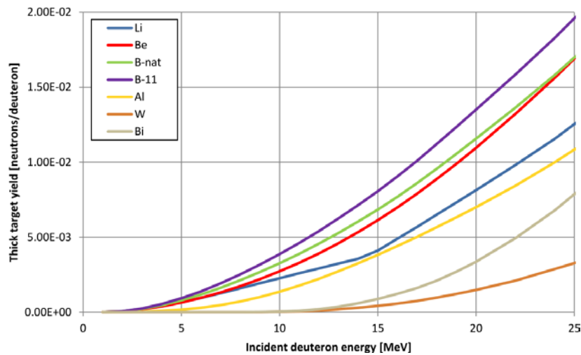
Fig. 2. Efficiency of different target materials for neutron yield as a function of the energy of deuterons.
