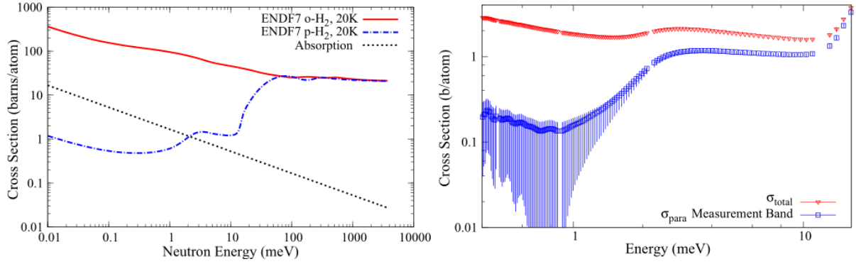
Fig. 11. Left: Scattering cross-sections for liquid ortho-H 2 (upper curve) and liquid para-H 2 (lower curve) from ENDF-VII. The para-H 2 is contaminated with a 0.5% admixture of ortho-H 2 . Right: Total cross section (including scattering and absorption) and scattering cross section of pure para-H 2 .
