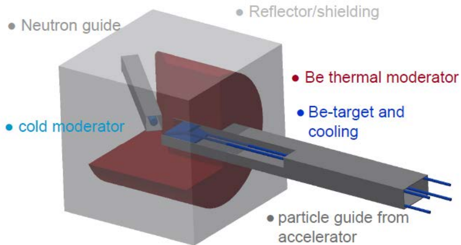
Fig. 5. Schematic drawing of a compact target-moderator setup with thermal and cold moderator
