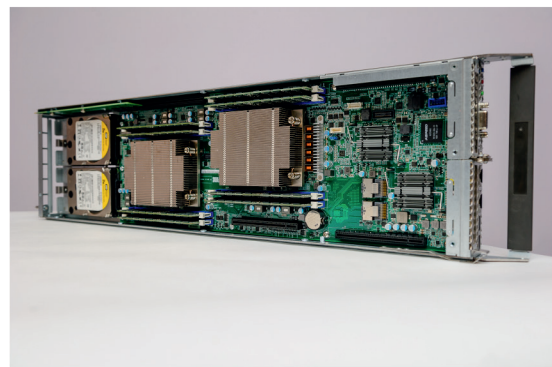
View of a T-Platforms V-Class V210S dual-socket blade server as used in JURECA.
